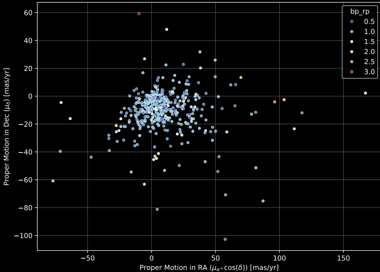
GALAH DR4 Field: [6688] Proper Motion Diagram (n= 412)
