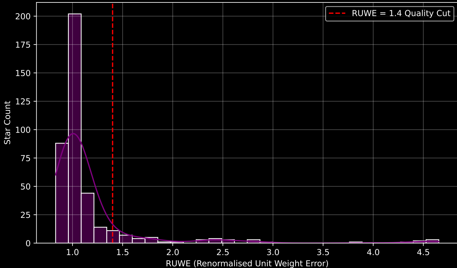
GALAH DR4 Field [6688] RUWE Distribution (n= 398)
