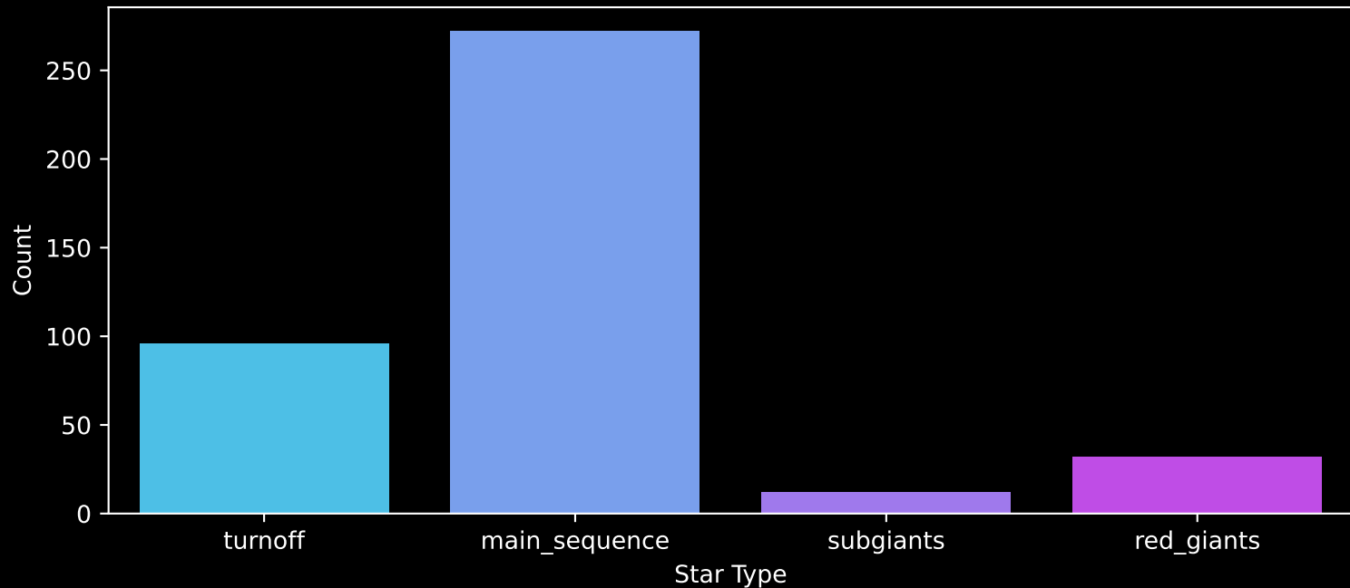
GALAH DR4 Field: [6688] Count plot of Star Type
