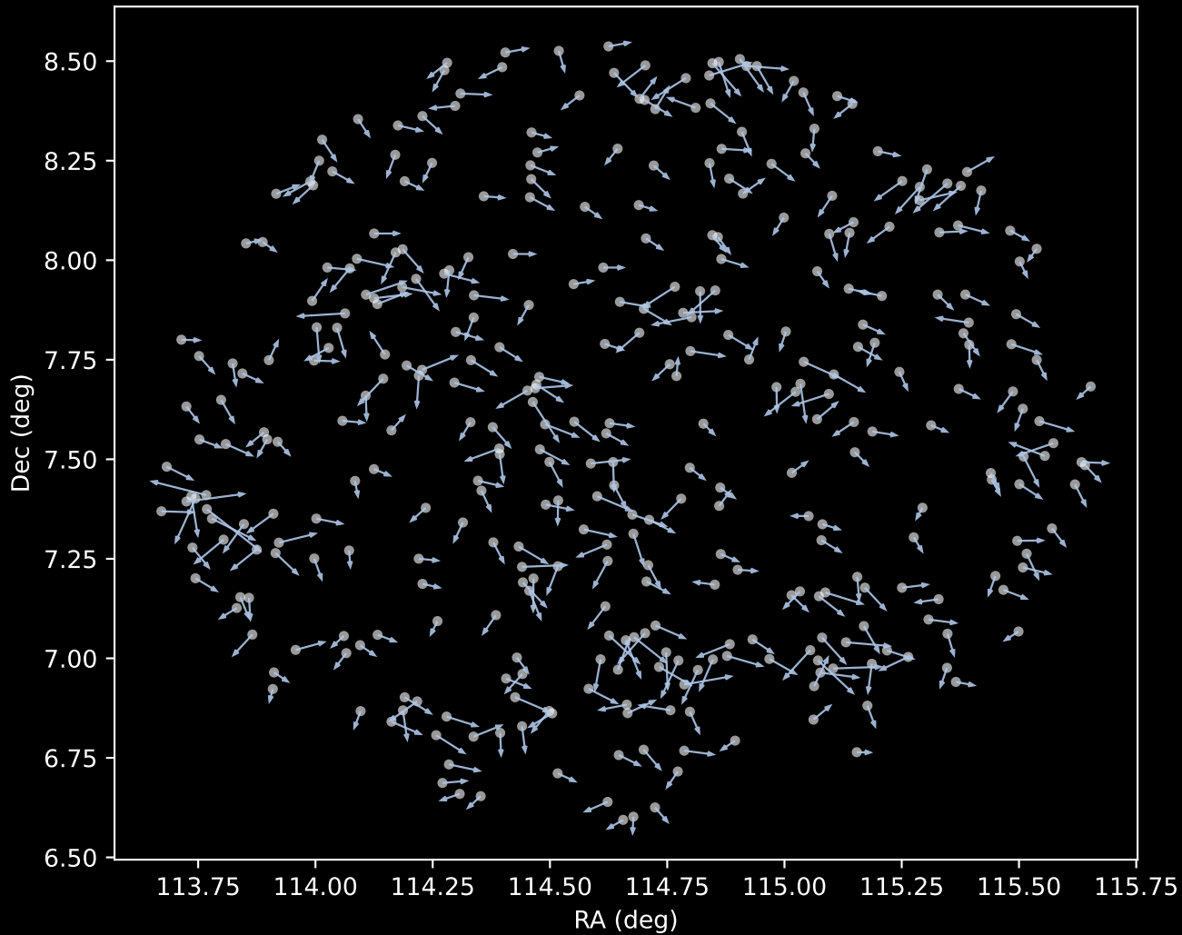
GALAH DR4 Cluster 1 Proper Motion Vectors (n=364)
